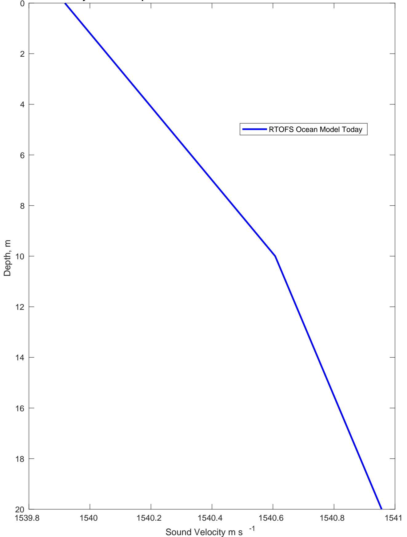
Sound Velocity Profile for SpaceX GOM Launch Platform on 07-Jul-2021 00:00:00
